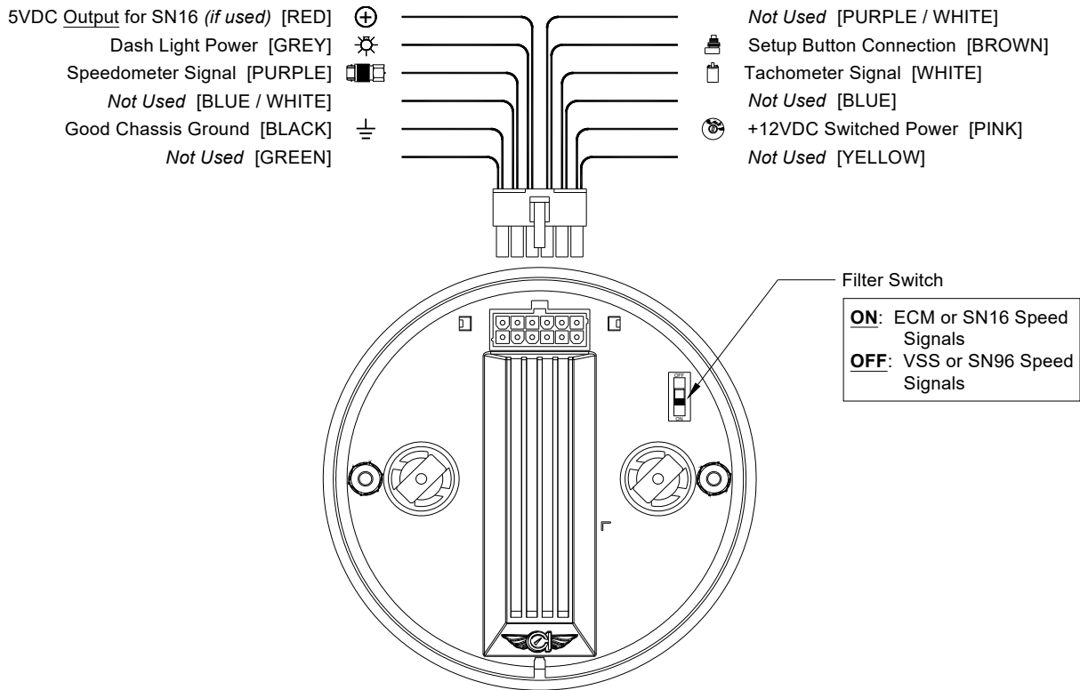
4 5/8" Speed-tachular Wiring
