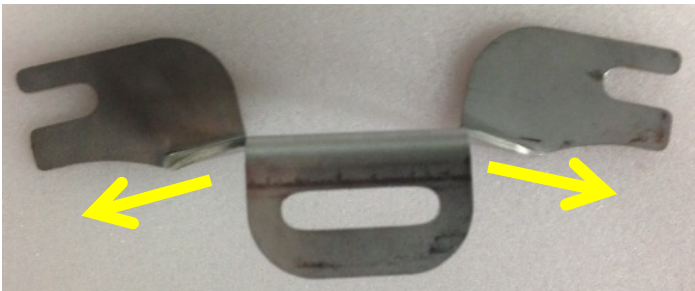
MTBRGMK – After Bending (Bend at thin sections)
